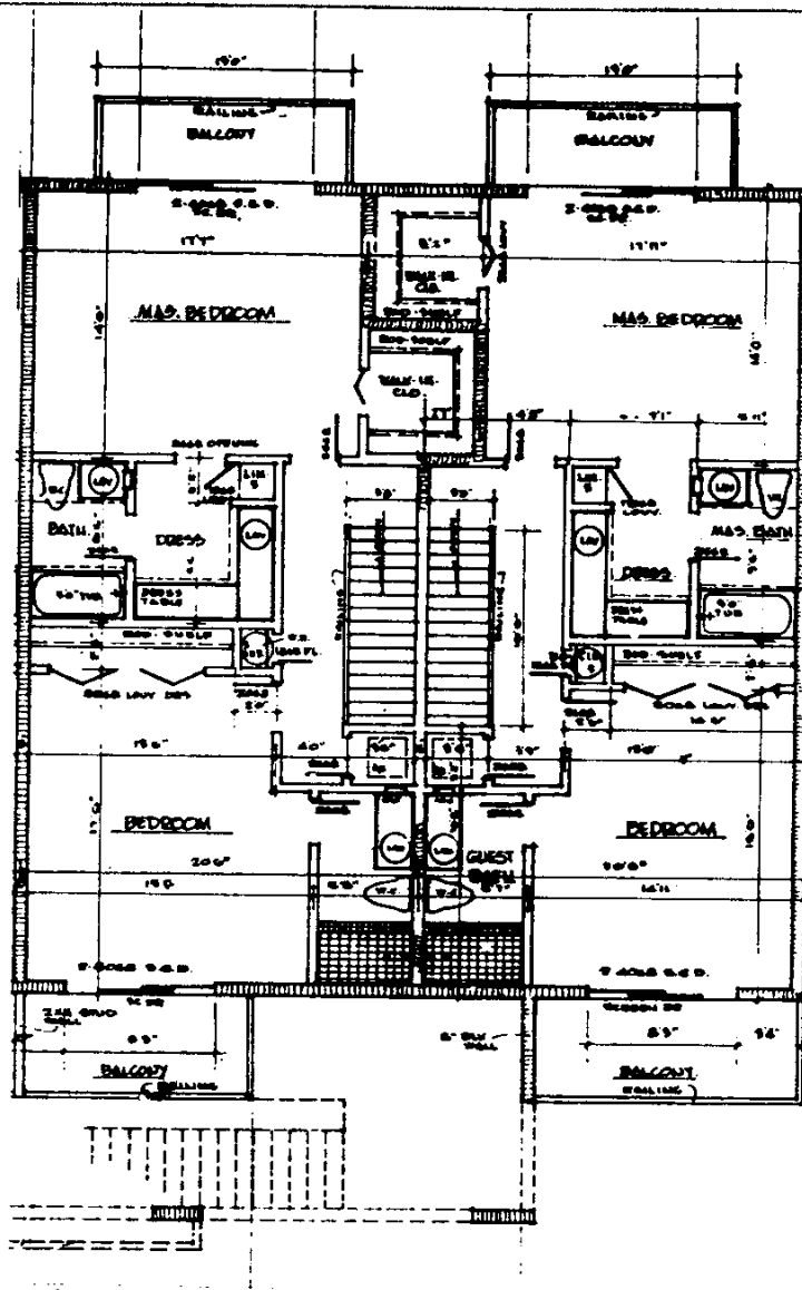
2nd Floor Townhouse Unit
