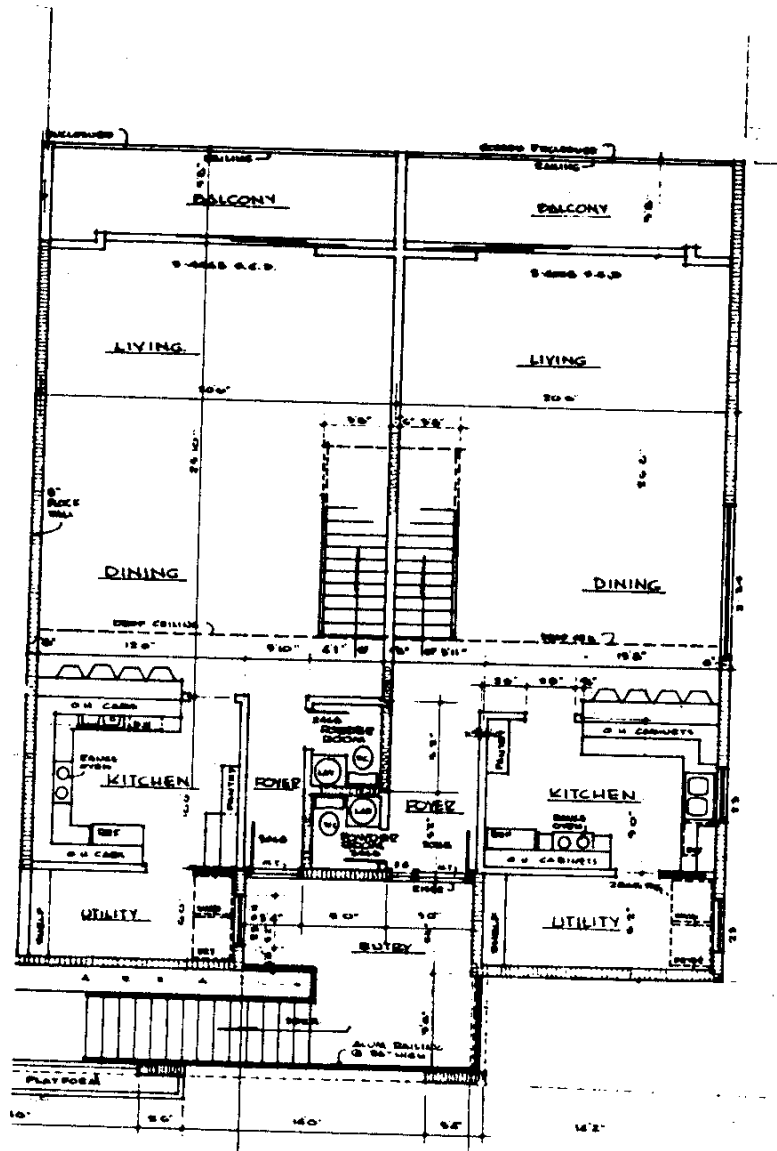
First Floor Townhouse Unit 2 Bedroom 2 Bath
