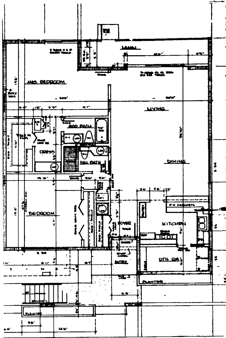
Ground Floor 2 Bedroom 2 Bath Apartment
