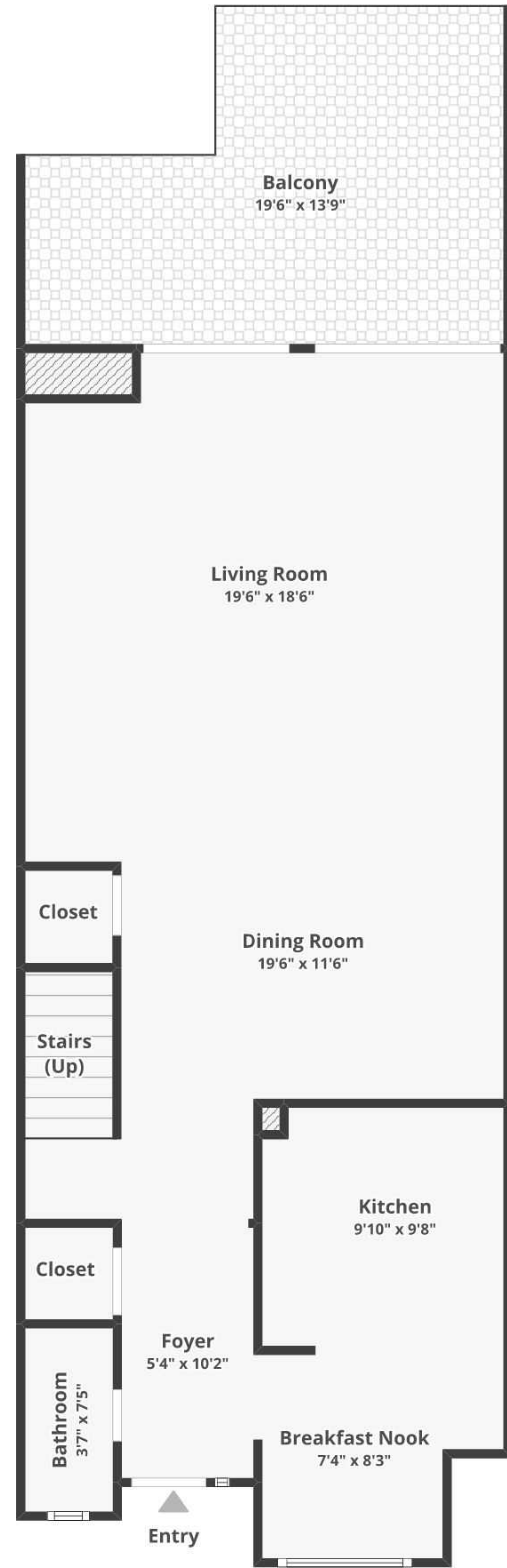
FLOOR 1
